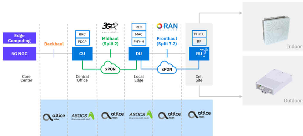
Figure 11: ASOCS-based indoor/outdoor infrastructure functional components
