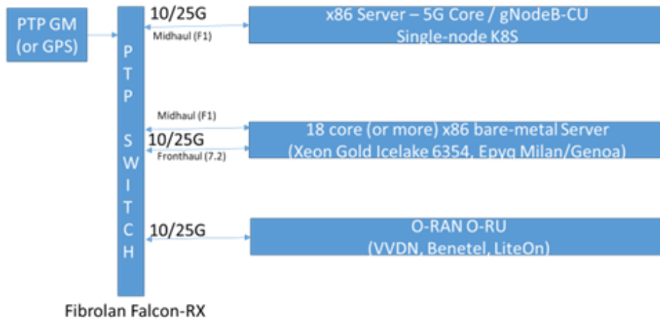
Figure 19(a): O-RAN equipment overview
