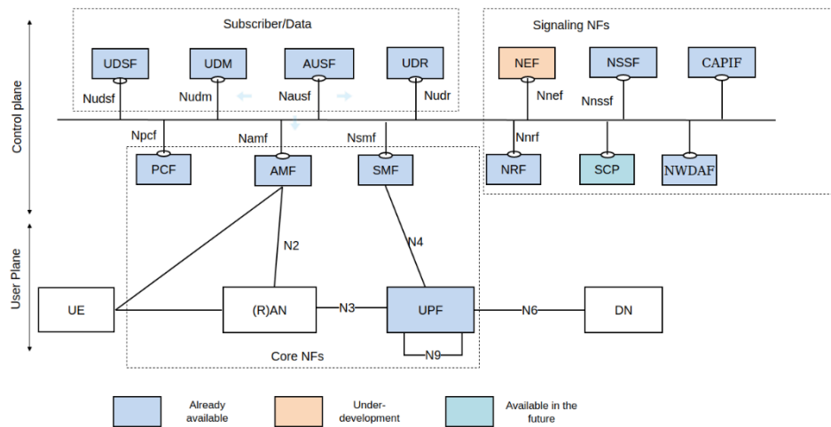
Figure 20: OAI 5G CN architecture
